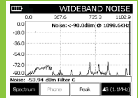
Wideband Noise
