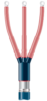
Heat-shrink termination, 3c paper MIND
